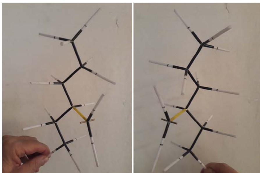
(S) -3-dihidroborexano (1) ↑ (R) -3-dihidroborexano (2) Enantiomeric products of hydroboration of cis -3-hexene ( S )-3-dihidroborexano and ( R )-3-dihidroborexano as specular images, Bravo et Vila, pp. 46-63
